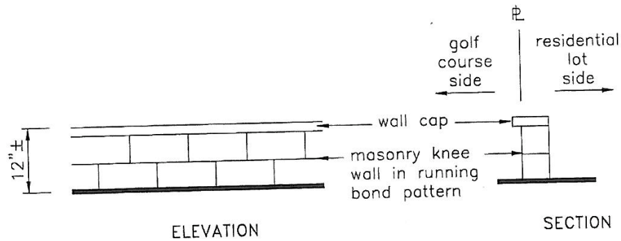
CONCEPTUAL KNEE WALL DETAIL
